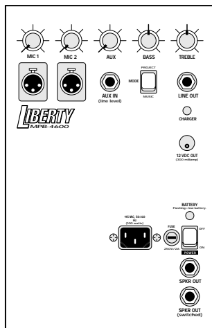
Liberty control panel.
